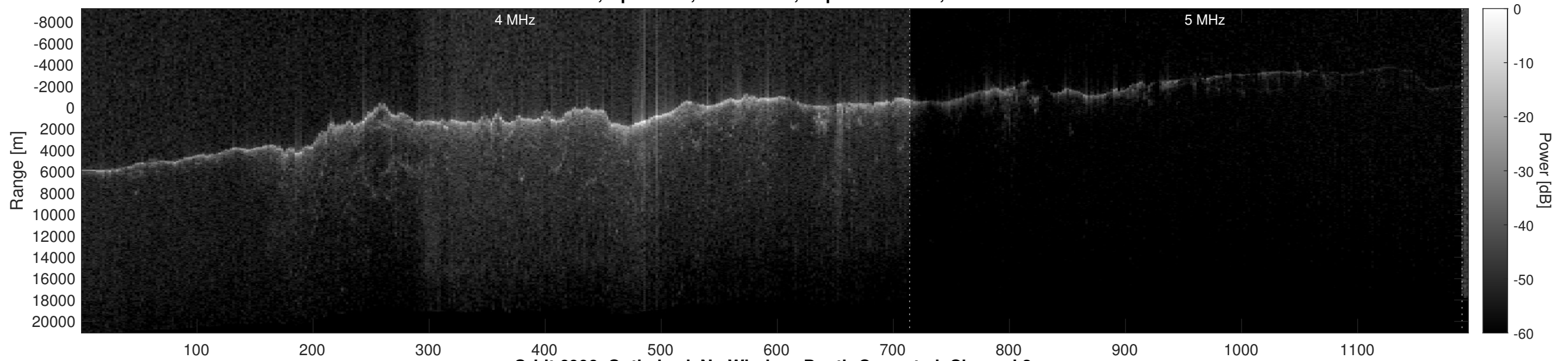
Orbit 6906, Optimized, No Window, Depth-Corrected, Channel 2
