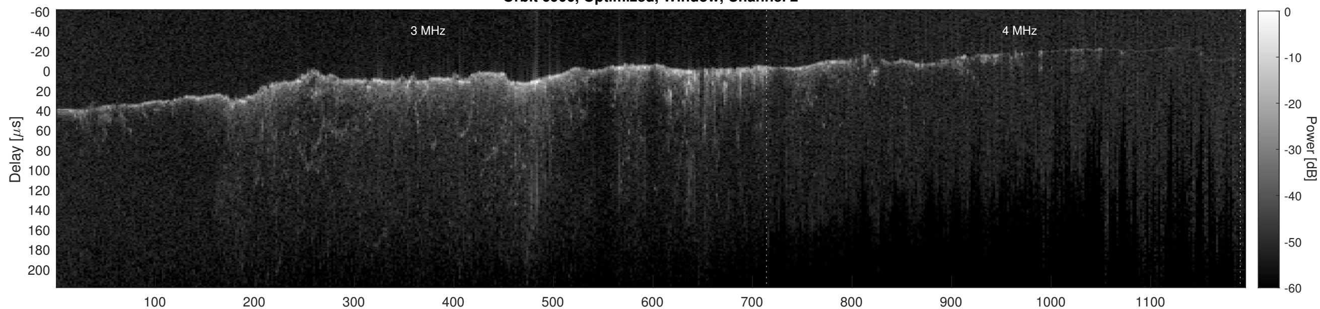
Orbit 6906, Cluttergram
