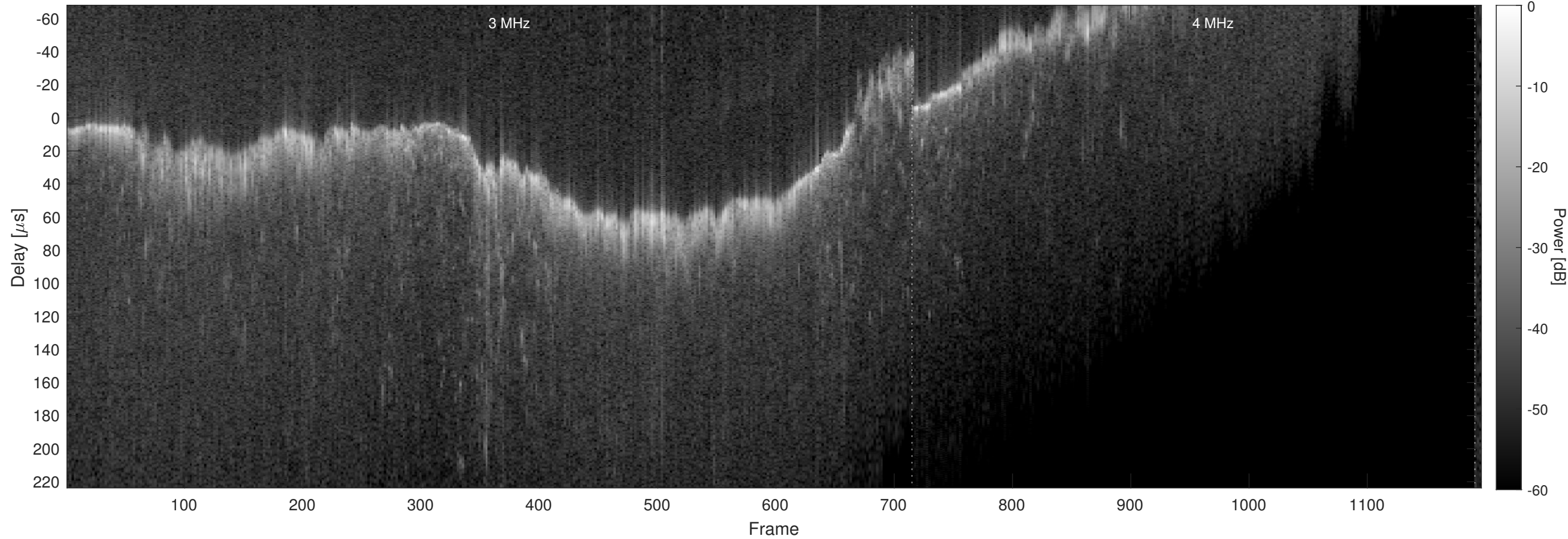
Orbit 6907, Chapman, No Window, Channel 2
