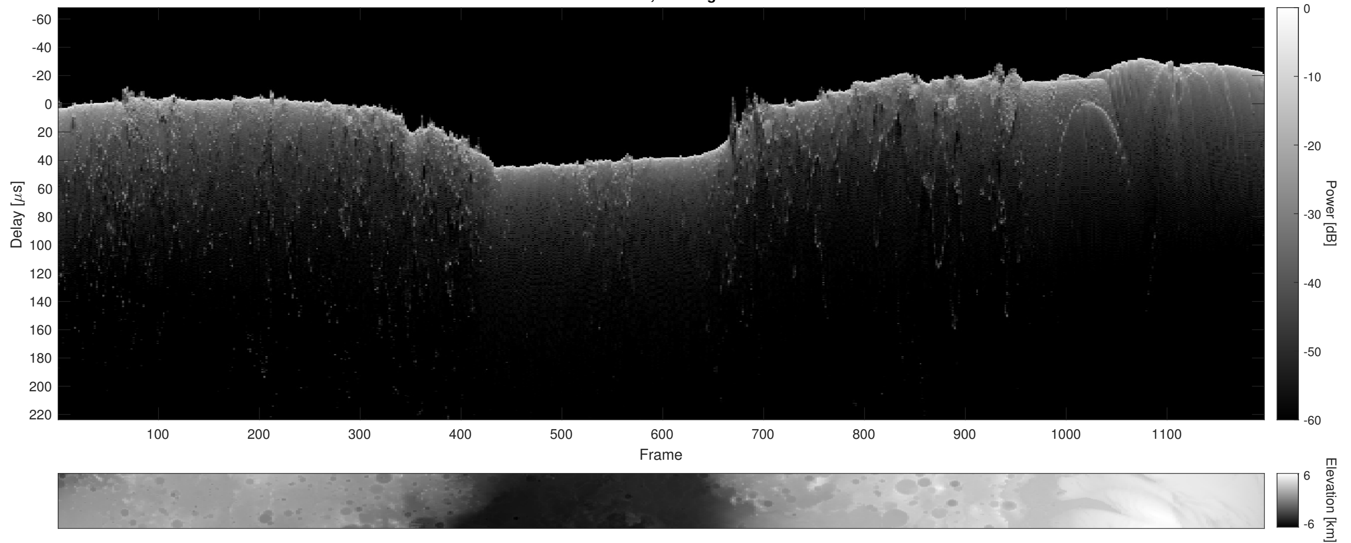
Orbit 6907, Cluttergram
