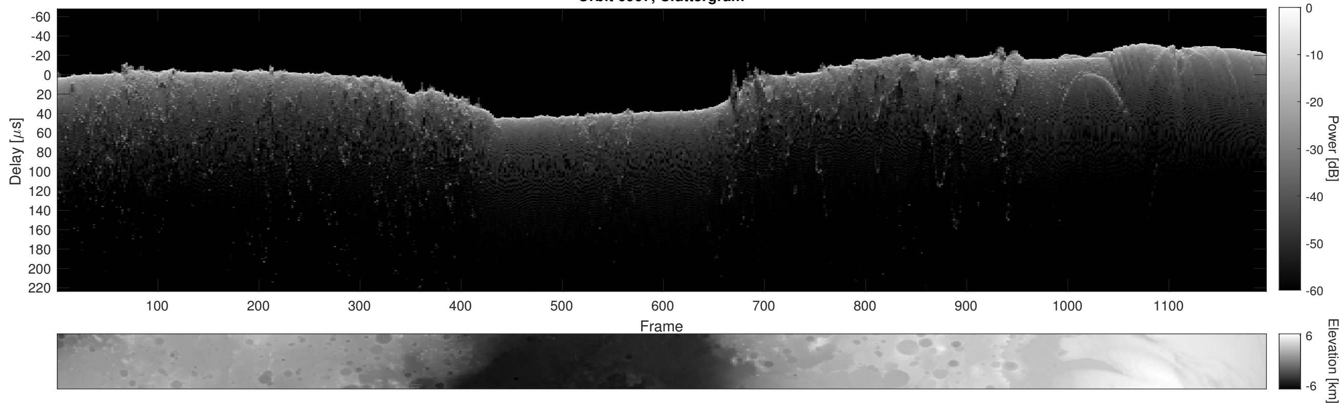
Orbit 6907, Cluttergram
