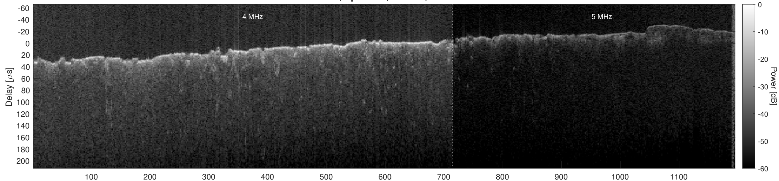
Orbit 6908, Optimized, Window, Channel 2
