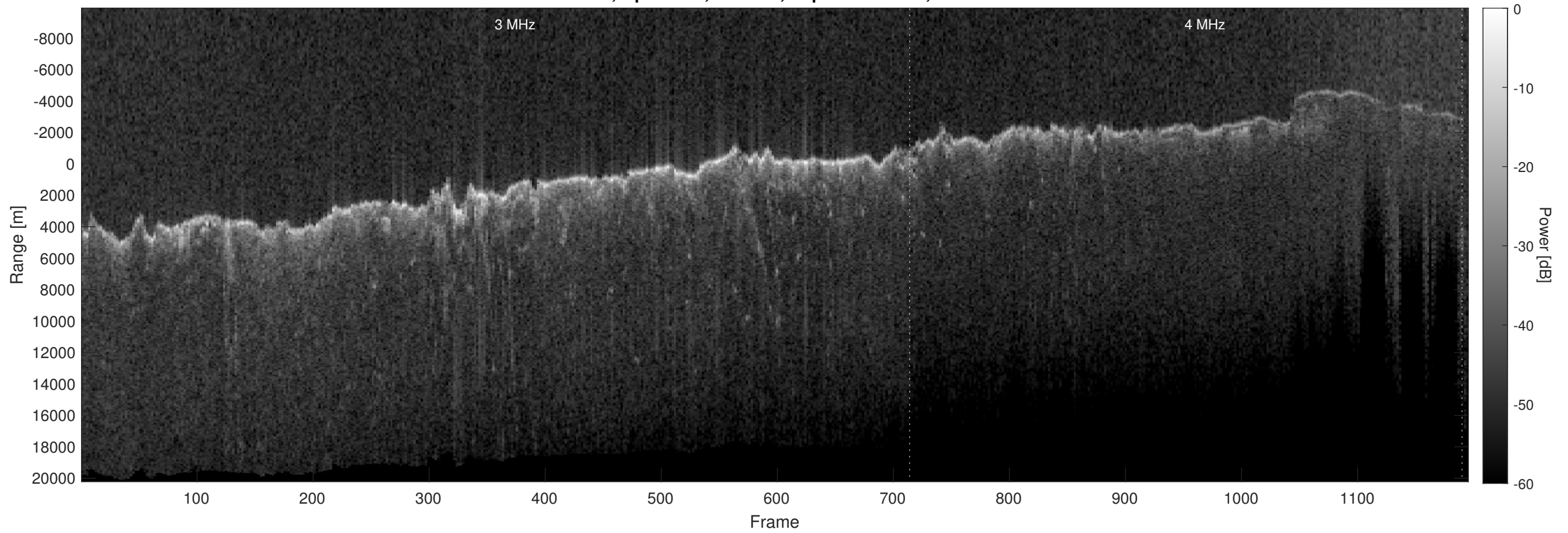
Orbit 6908, Optimized, Window, Depth-Corrected, Channel 2
