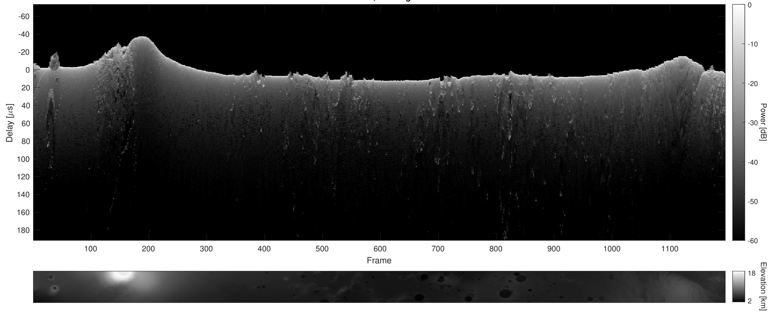
Orbit 6909, Cluttergram
