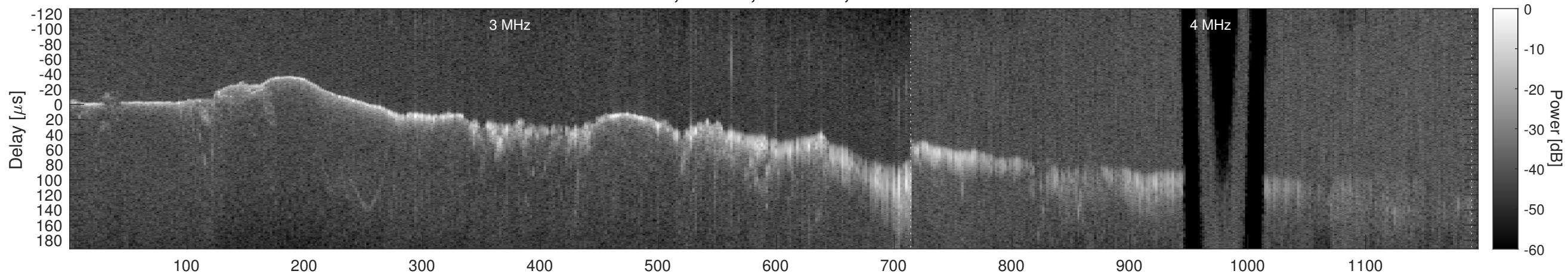
Orbit 6909, Window, Channel 2, Chapman
