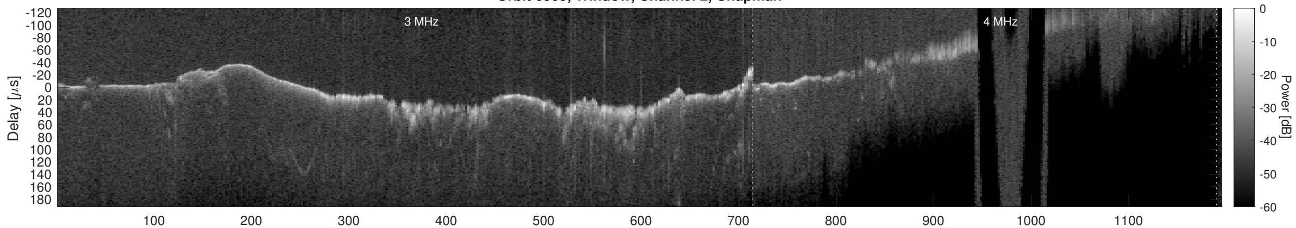
Orbit 6909, Window, Channel 2, Optimized
