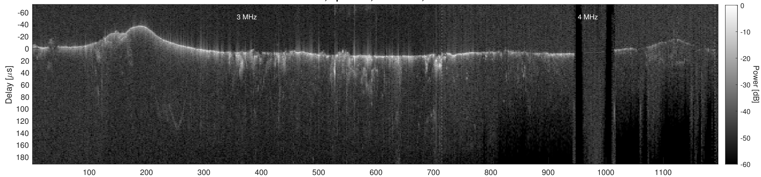
Orbit 6909, Cluttergram
