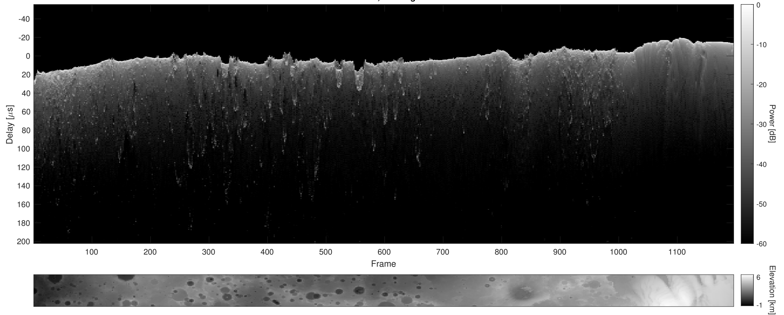
Orbit 6911, Cluttergram
