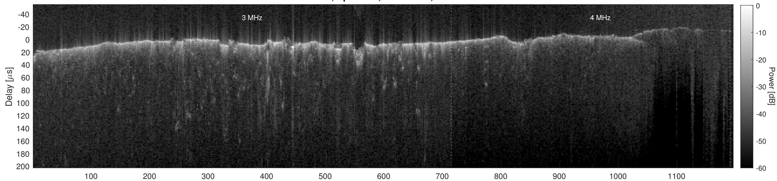
Orbit 6911, Cluttergram
