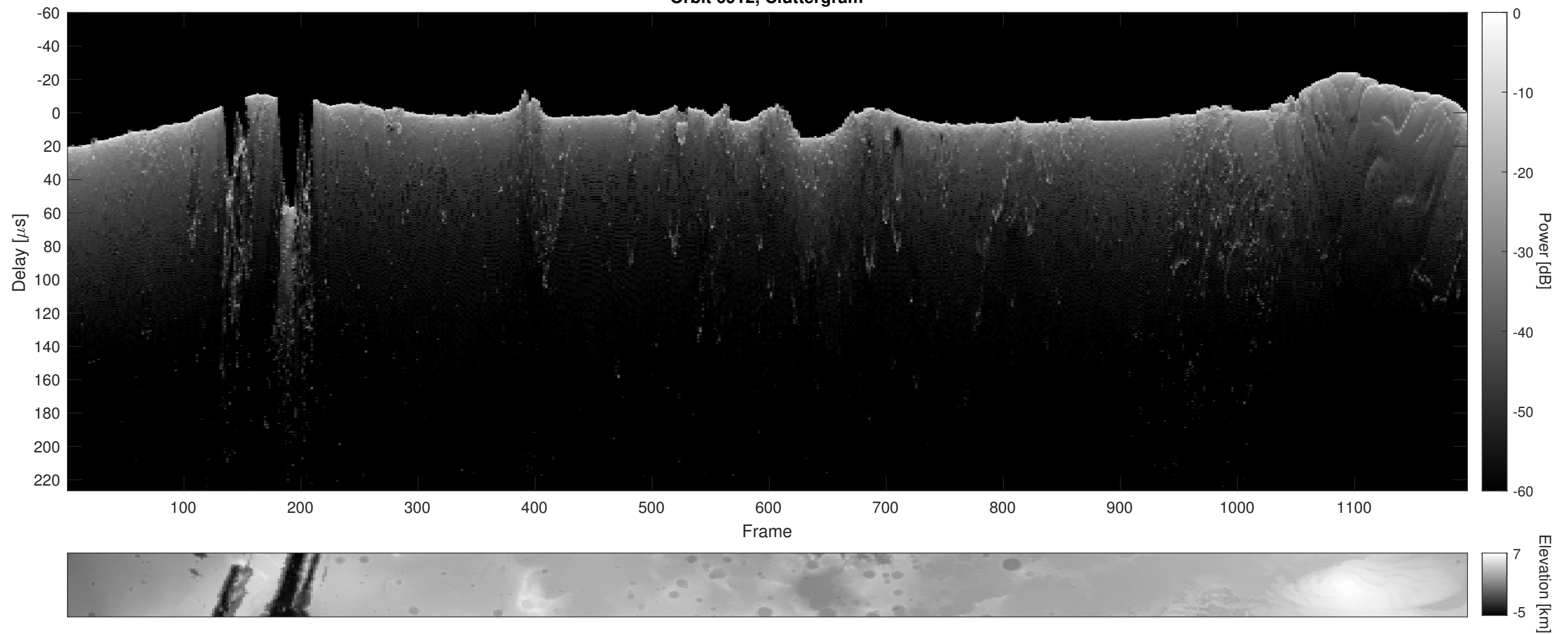
Orbit 6912, Cluttergram
