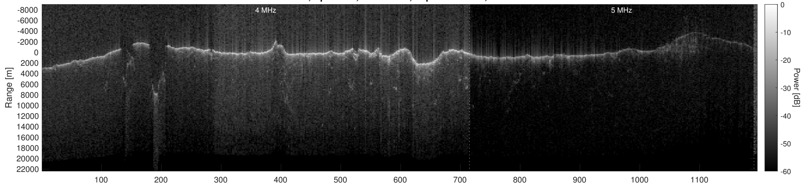
Orbit 6912, Optimized, No Window, Depth-Corrected, Channel 2
