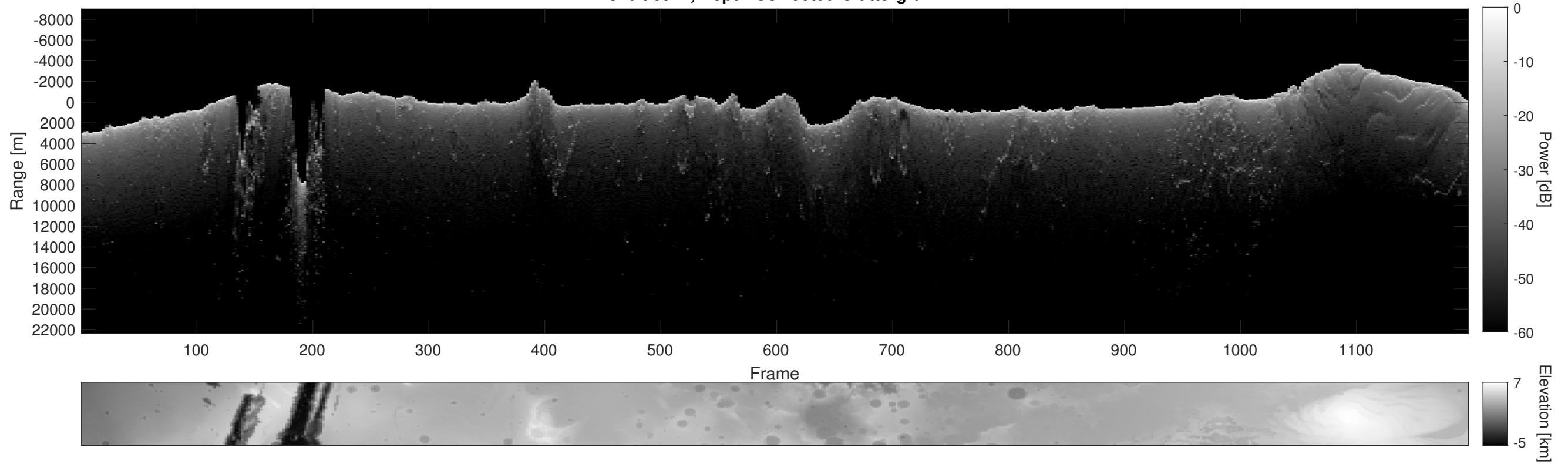
Orbit 6912, Depth-Corrected Cluttergram
