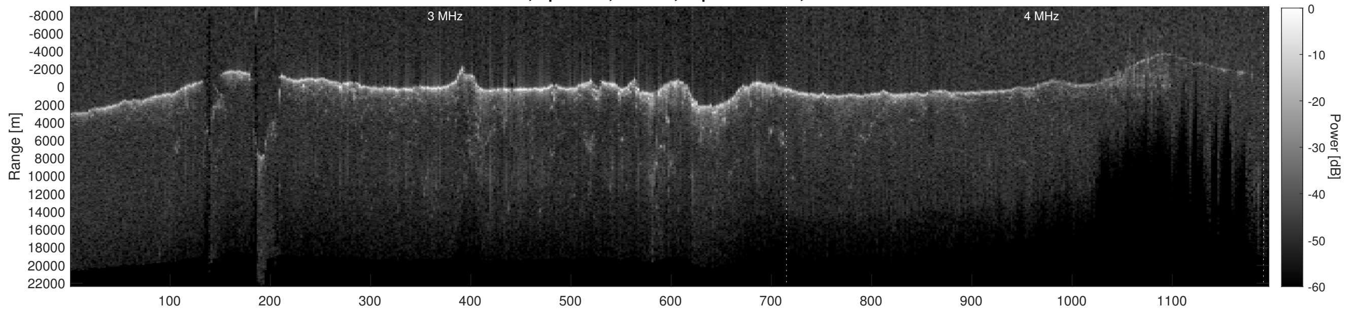
Orbit 6912, Depth-Corrected Cluttergram
