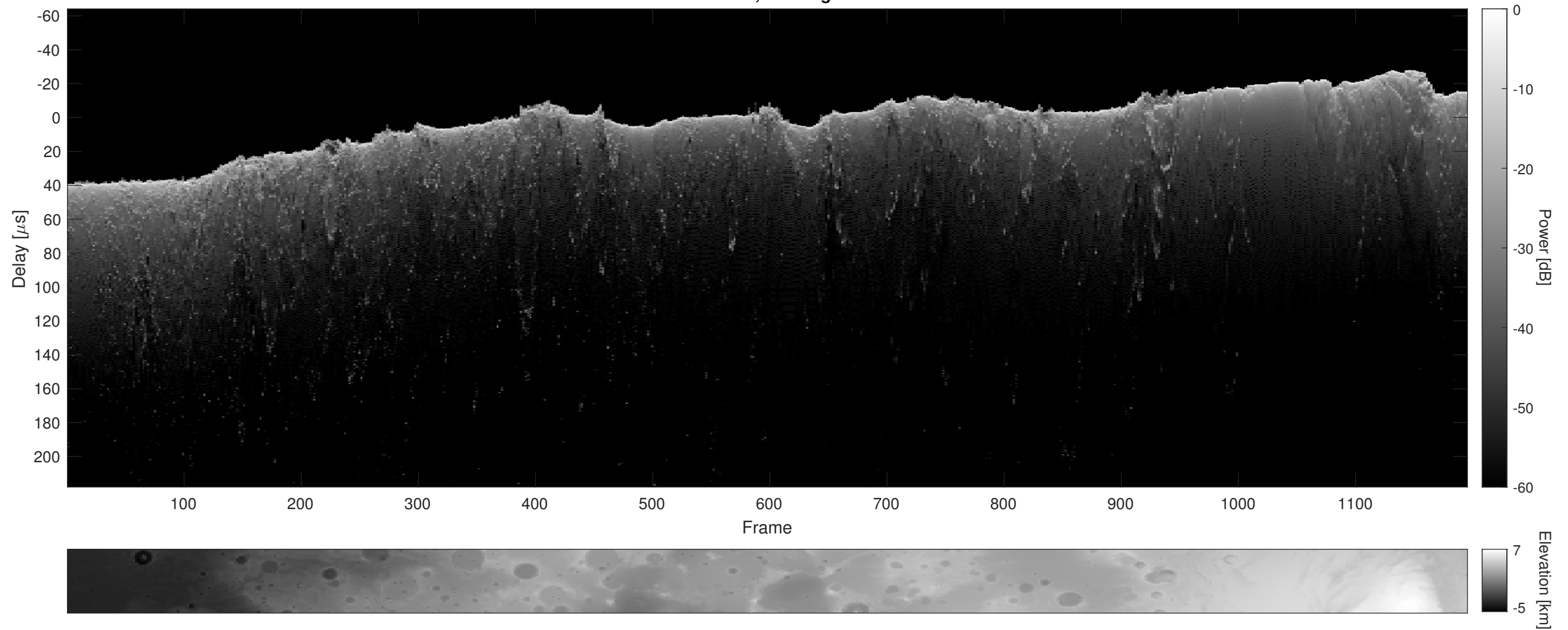
Orbit 6913, Cluttergram
