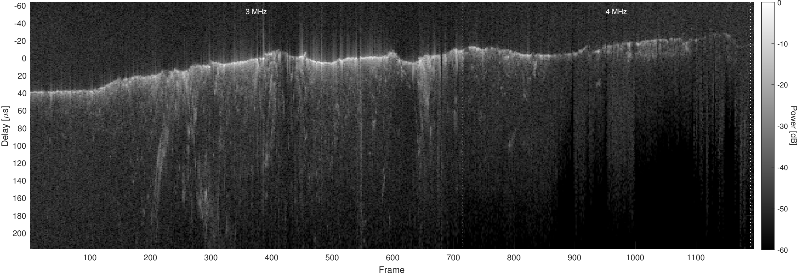
Orbit 6913, Optimized, No Window, Channel 2
