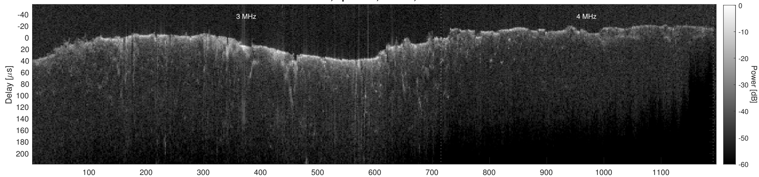
Orbit 6914, Cluttergram
