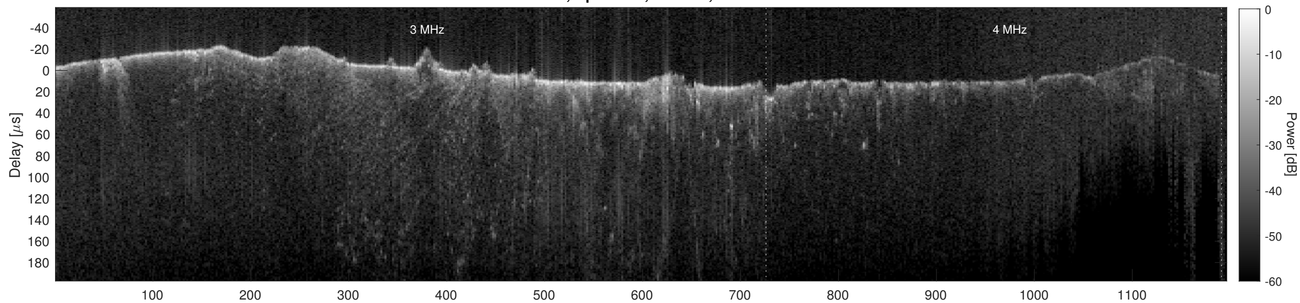
Orbit 6916, Cluttergram
