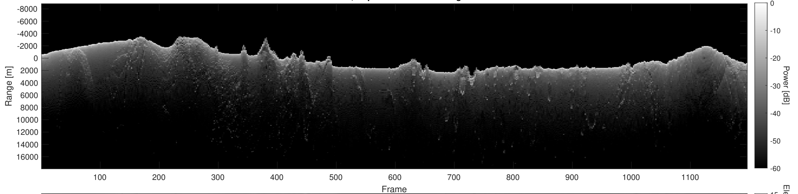
Orbit 6916, Depth-Corrected Cluttergram
