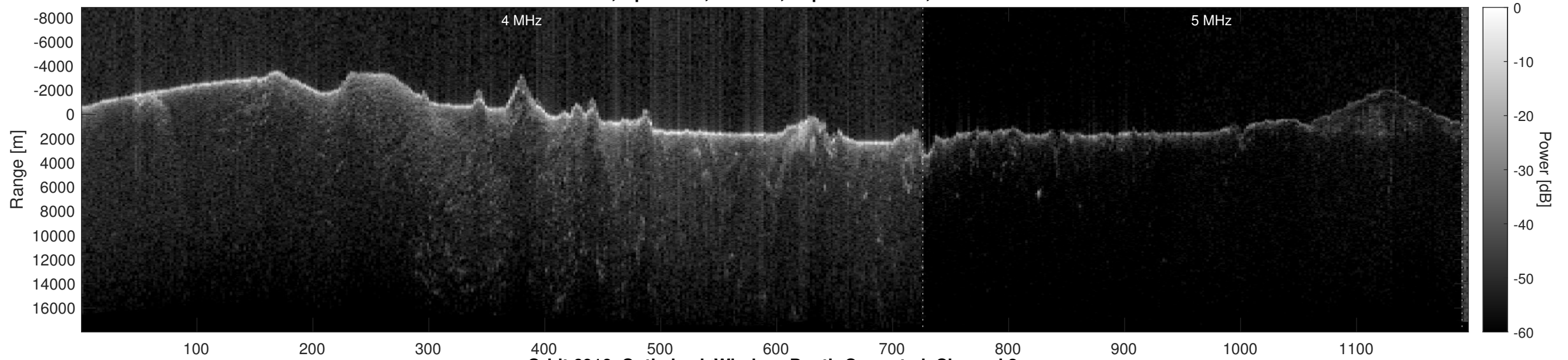
Orbit 6916, Optimized, Window, Depth-Corrected, Channel 2
