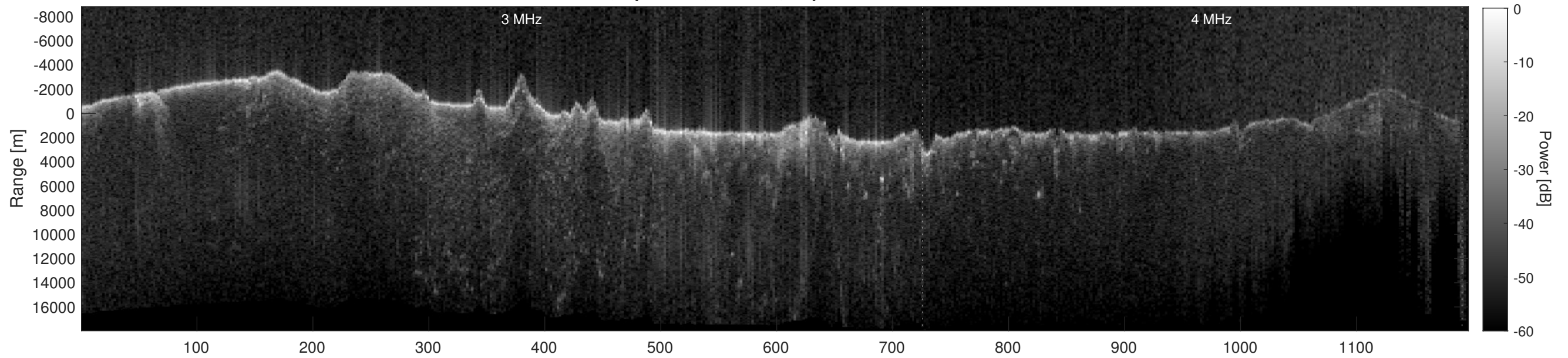
Orbit 6916, Depth-Corrected Cluttergram
