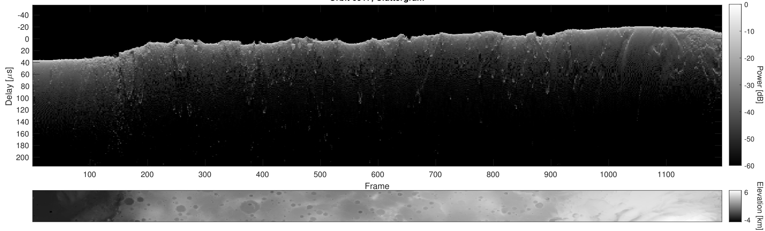
Orbit 6917, Cluttergram
