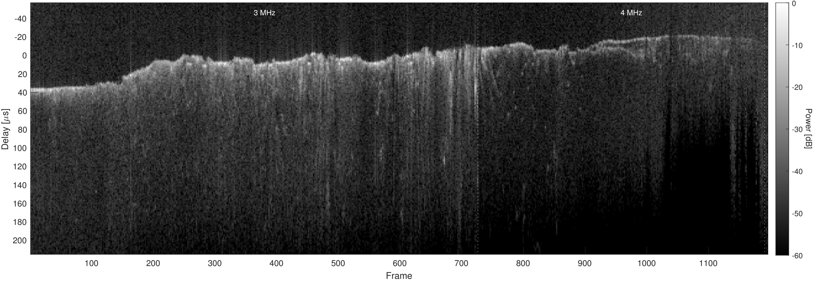
Orbit 6917, Optimized, Window, Channel 2
