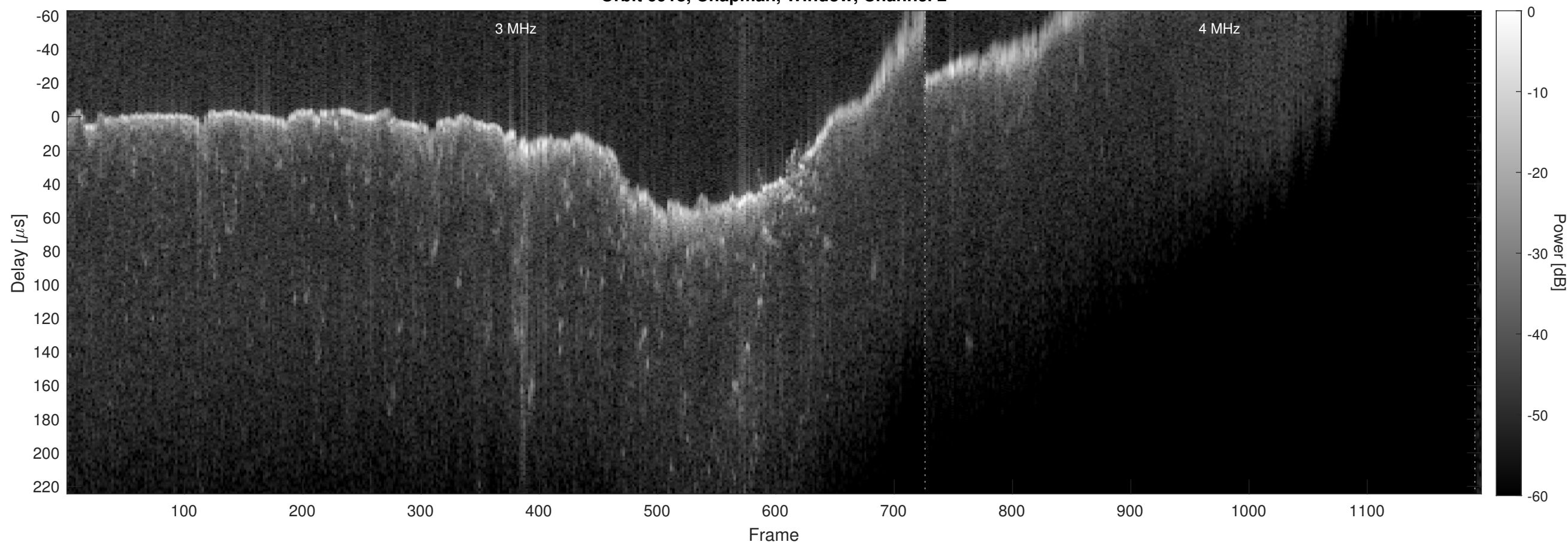
Orbit 6918, Chapman, Window, Channel 2
