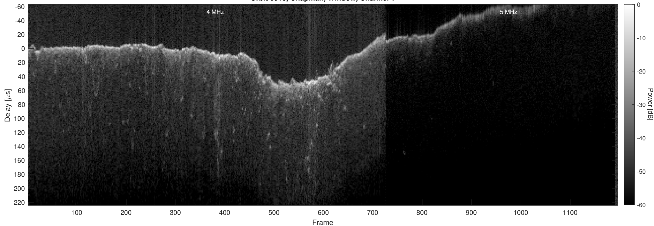
Orbit 6918, Chapman, Window, Channel 2
