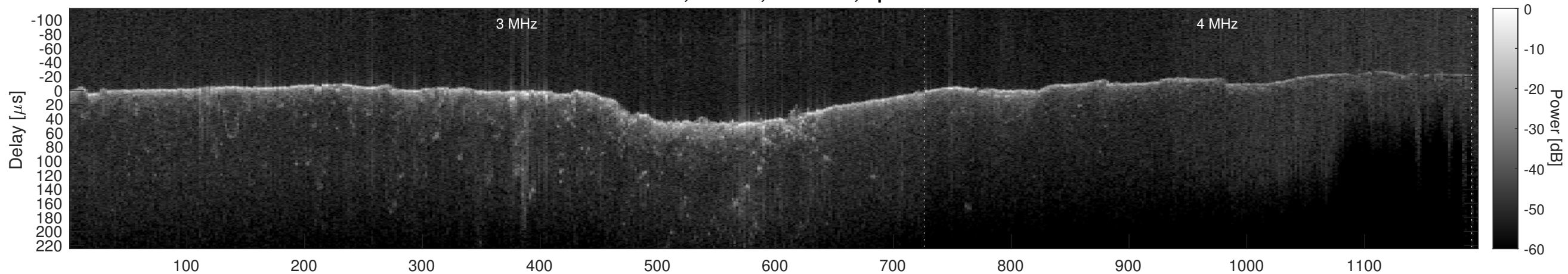
Orbit 6918, Cluttergram
