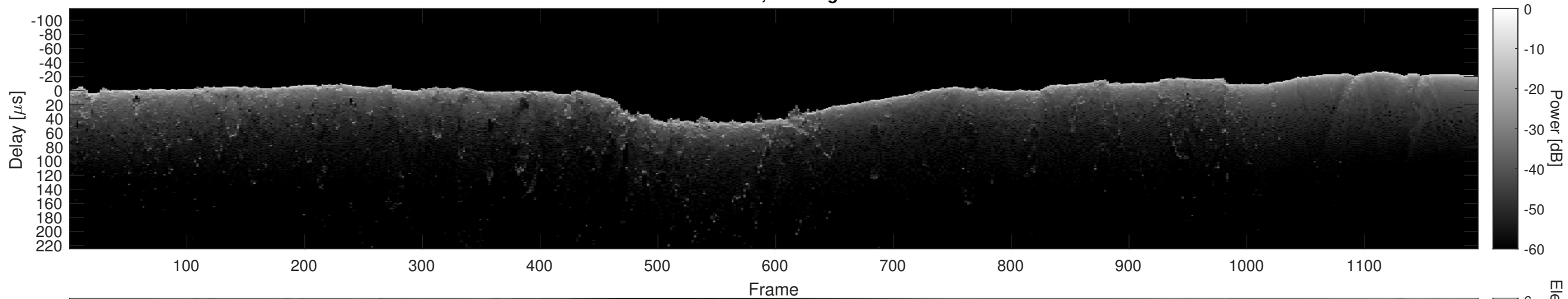
Orbit 6918, Cluttergram
