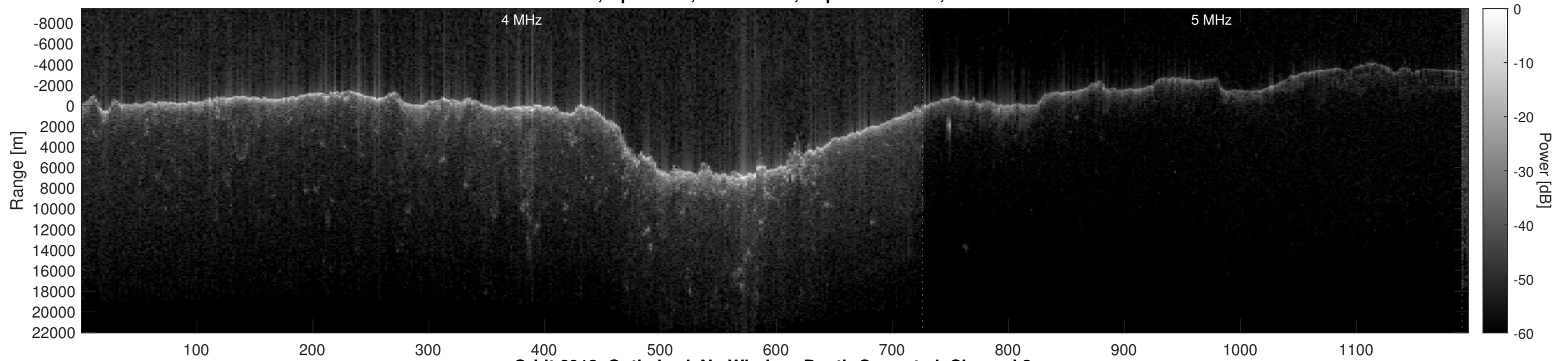
Orbit 6918, Optimized, No Window, Depth-Corrected, Channel 2
