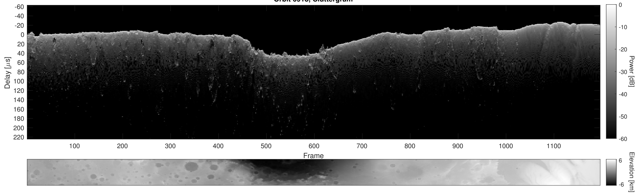
Orbit 6918, Cluttergram
