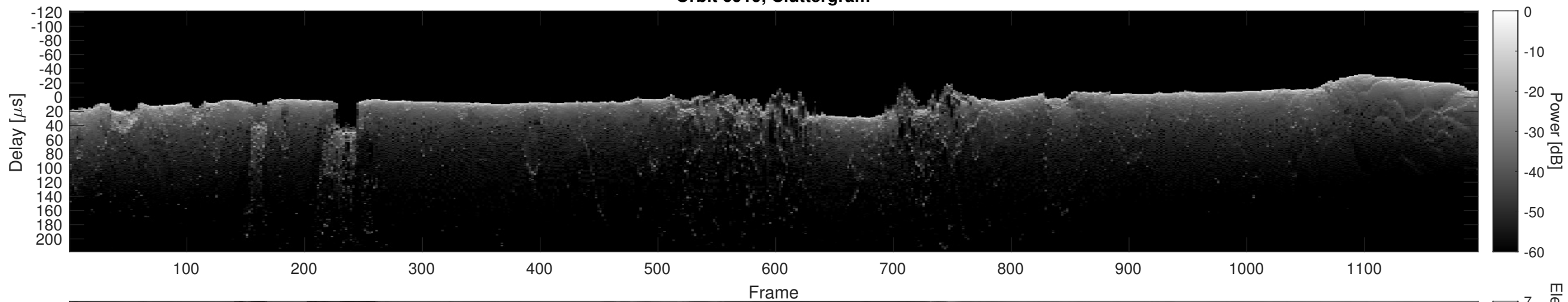
Orbit 6919, Cluttergram
