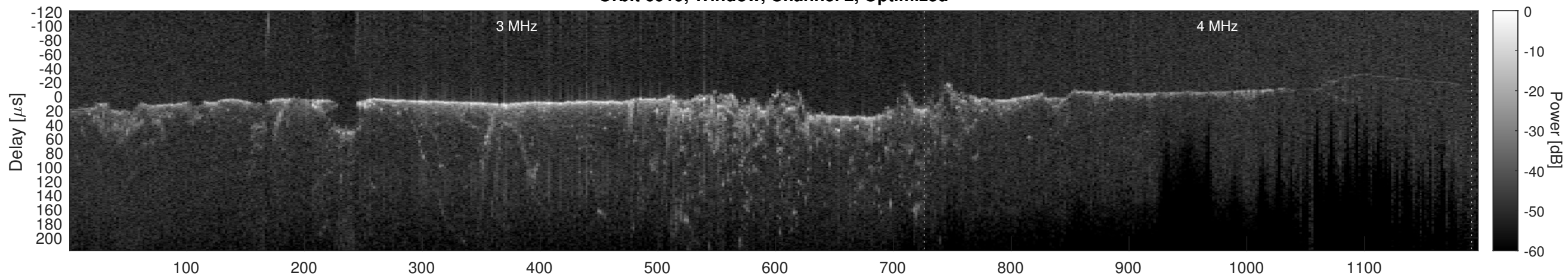
Orbit 6919, Cluttergram
