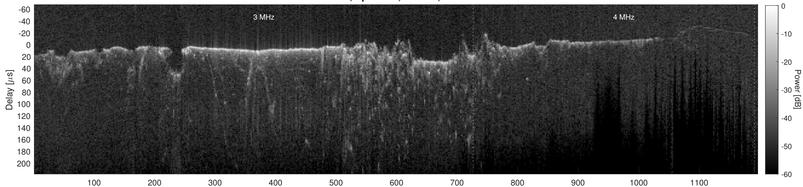
Orbit 6919, Cluttergram
