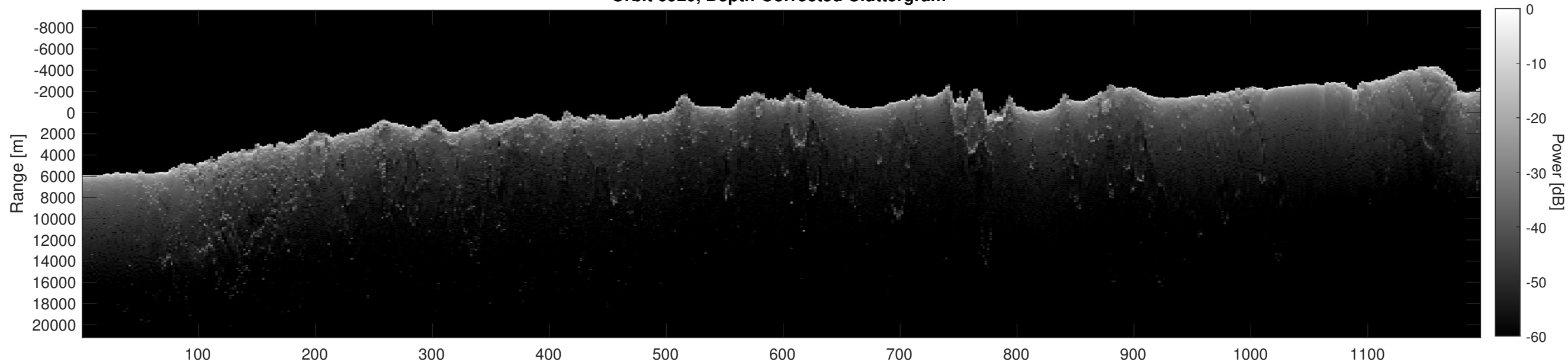
Orbit 6920, Depth-Corrected Cluttergram
