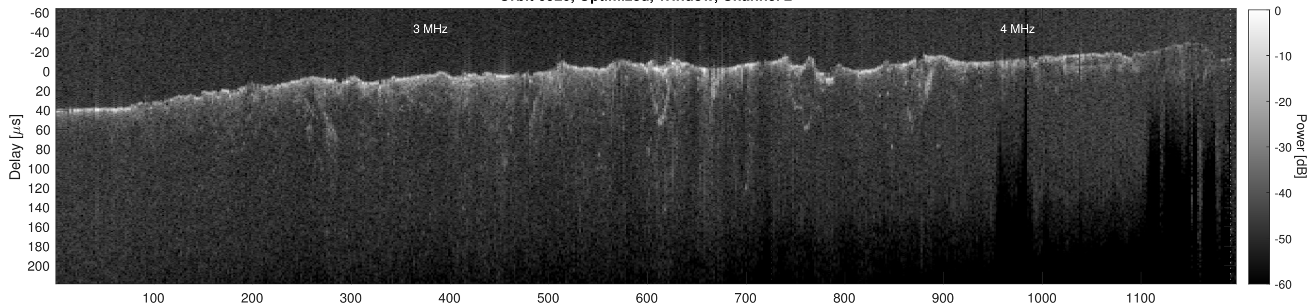
Orbit 6920, Cluttergram
