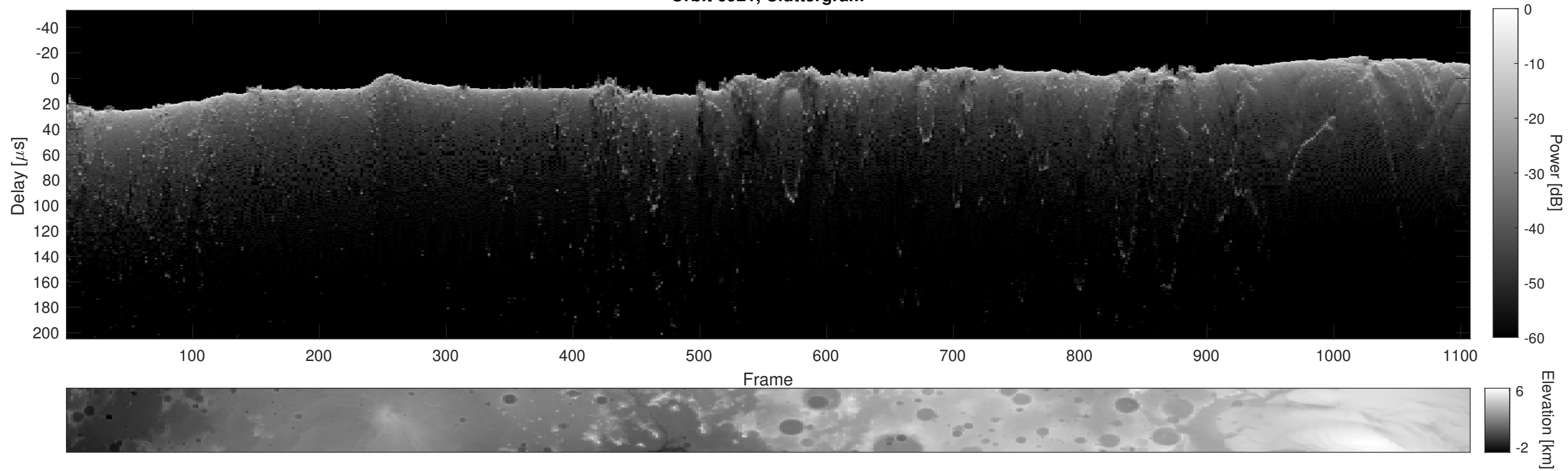
Orbit 6921, Cluttergram
