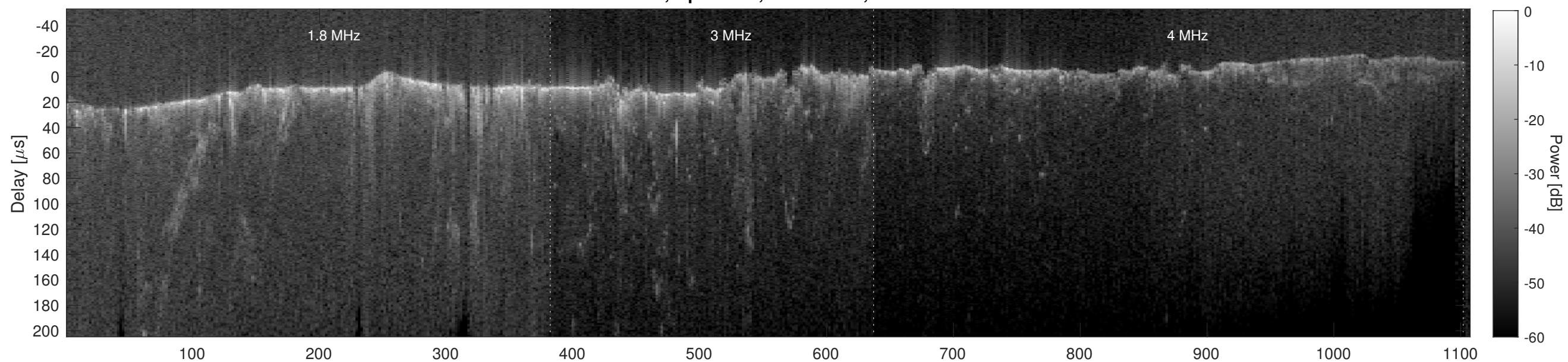
Orbit 6921, Cluttergram
