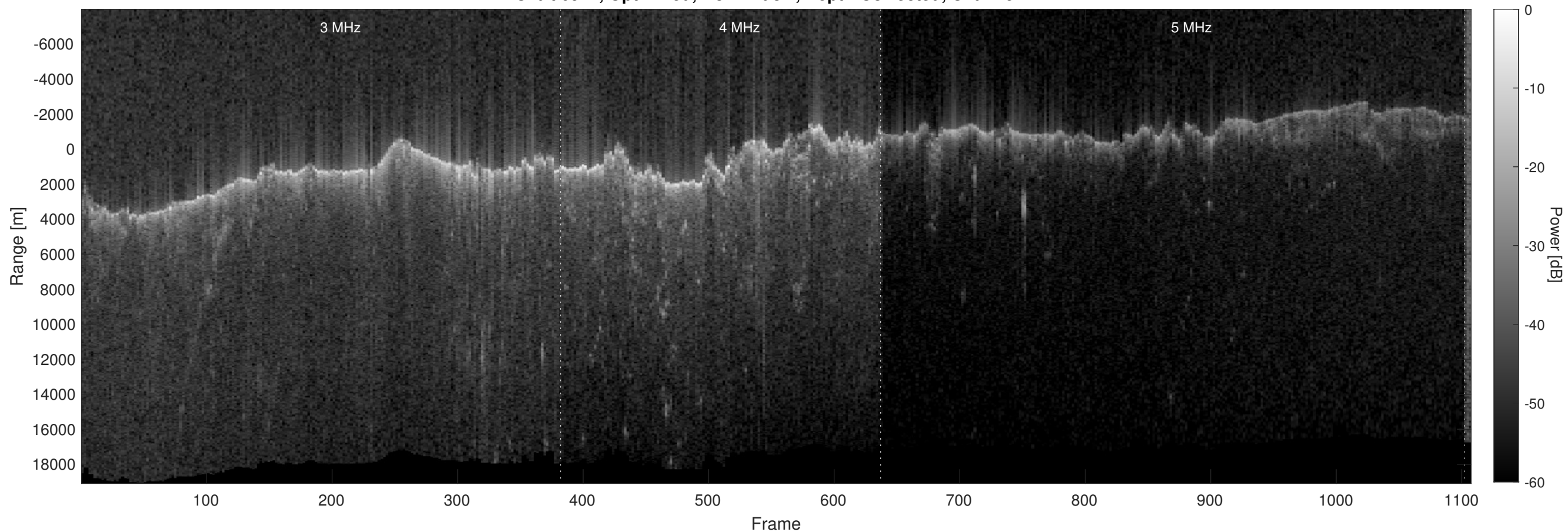
Orbit 6921, Optimized, No Window, Depth-Corrected, Channel 2
