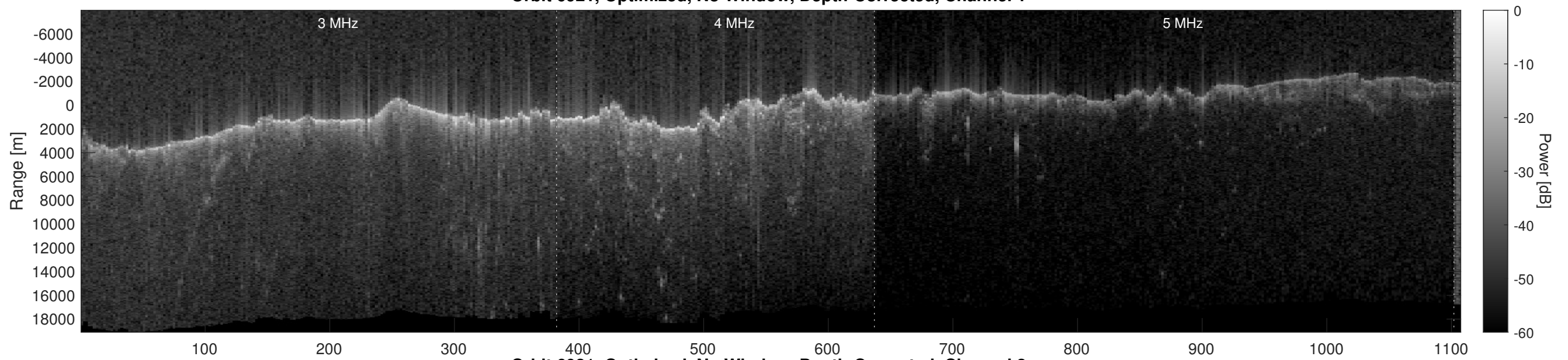
Orbit 6921, Optimized, No Window, Depth-Corrected, Channel 2
