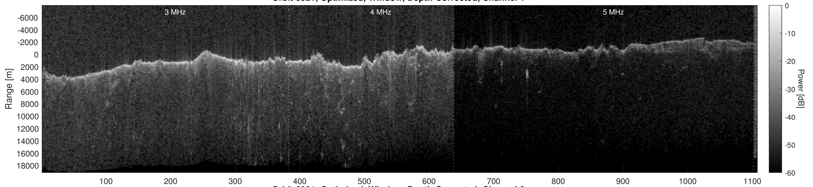
Orbit 6921, Optimized, Window, Depth-Corrected, Channel 2
