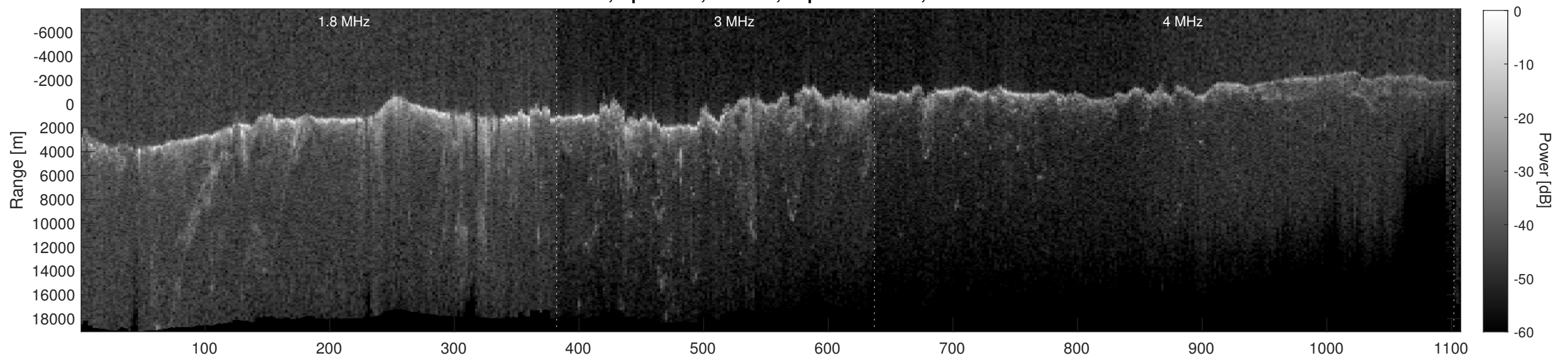
Orbit 6921, Depth-Corrected Cluttergram
