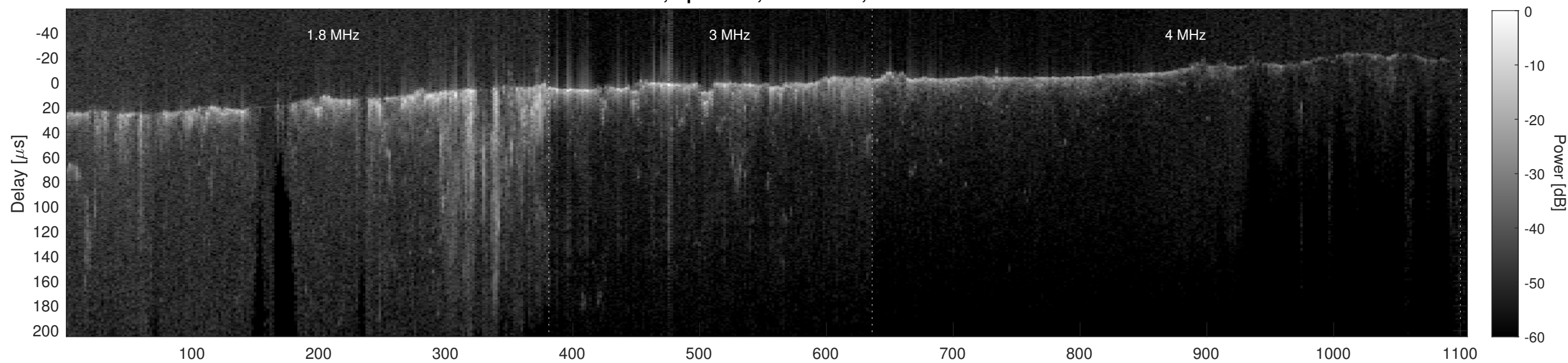
Orbit 6922, Cluttergram
