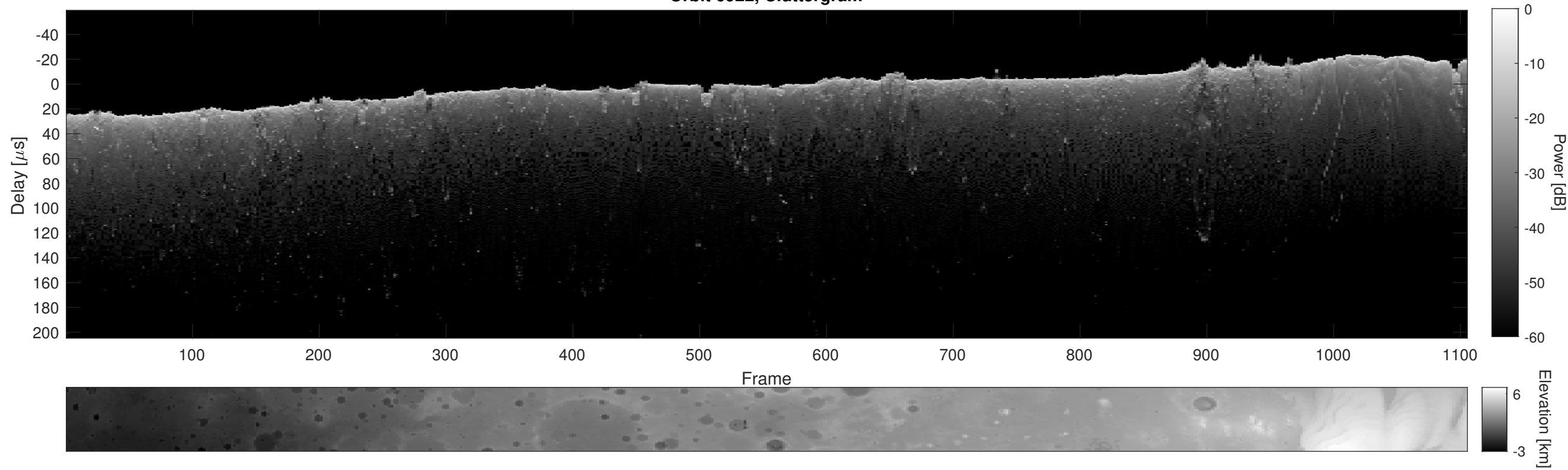
Orbit 6922, Cluttergram
