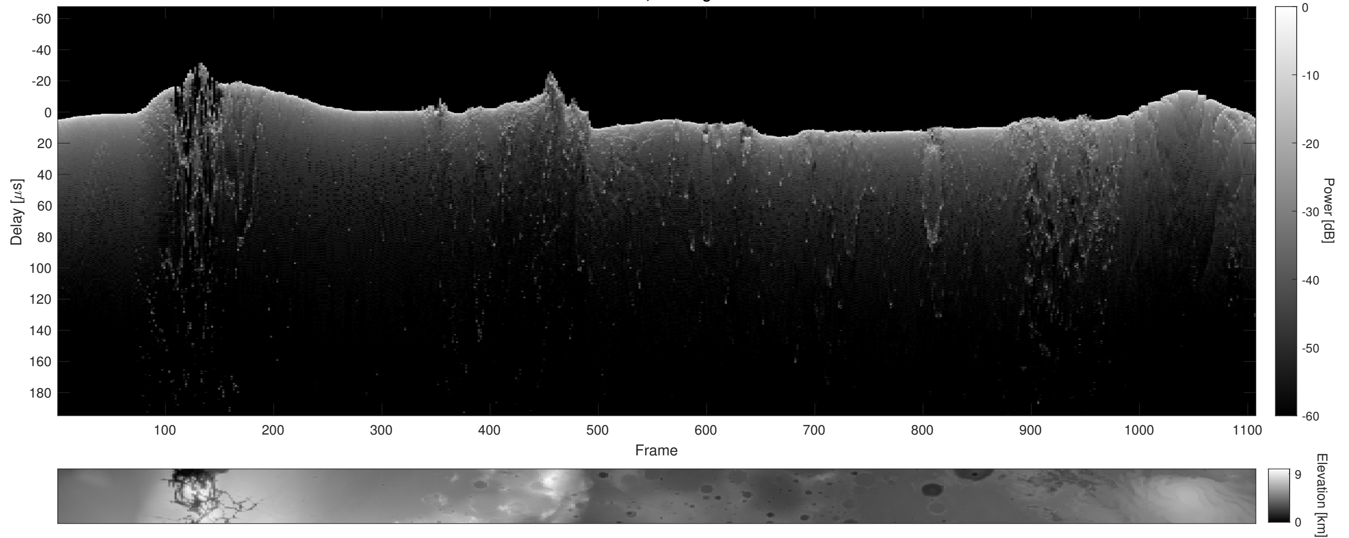
Orbit 6923, Cluttergram
