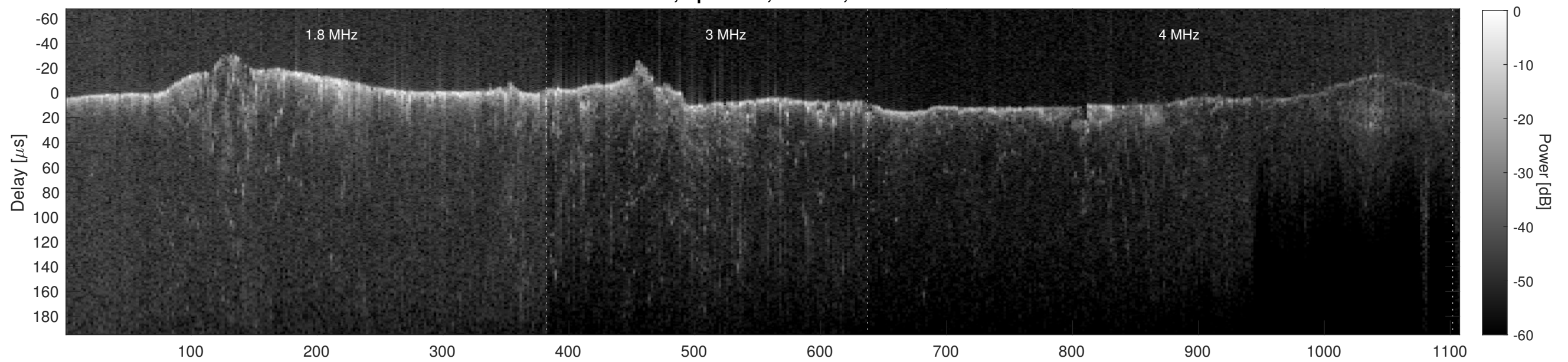
Orbit 6923, Cluttergram
