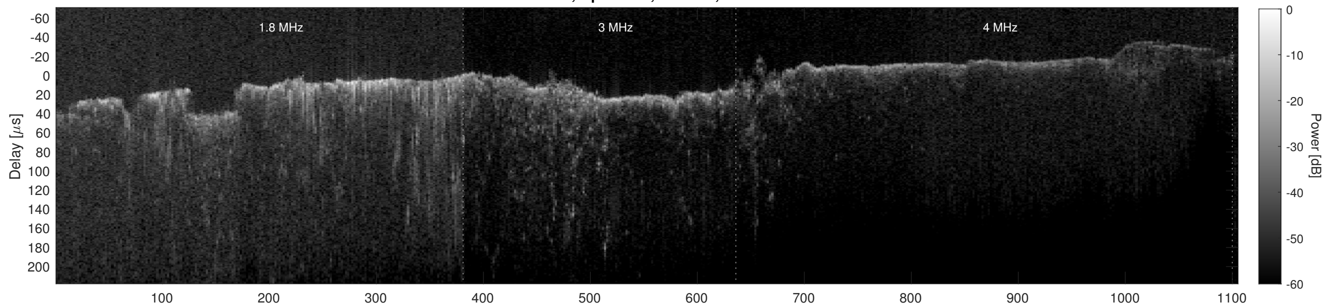
Orbit 6926, Cluttergram
