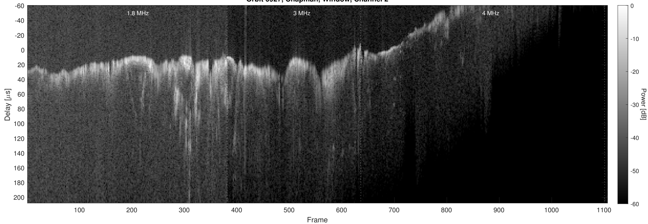
Orbit 6927, Chapman, Window, Channel 2
