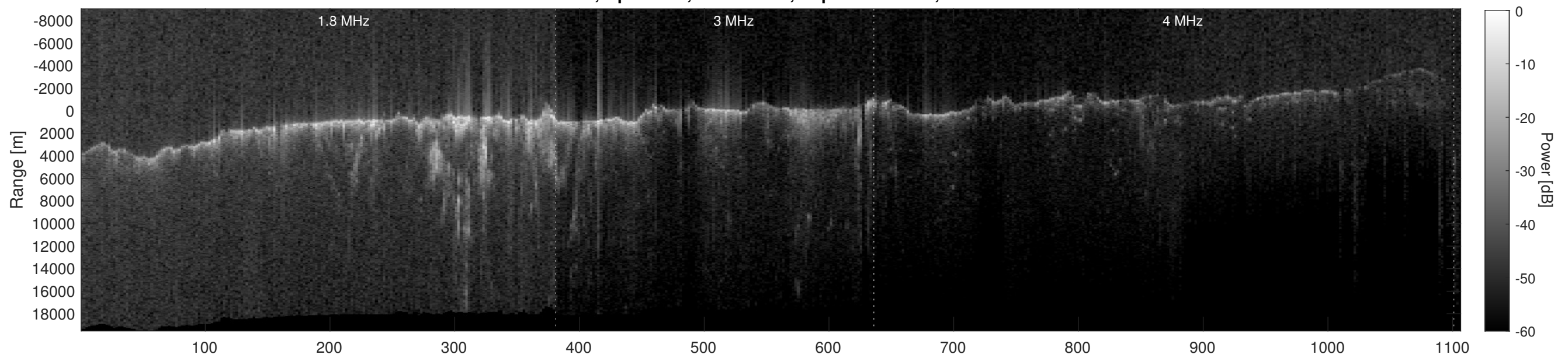
Orbit 6927, Depth-Corrected Cluttergram
