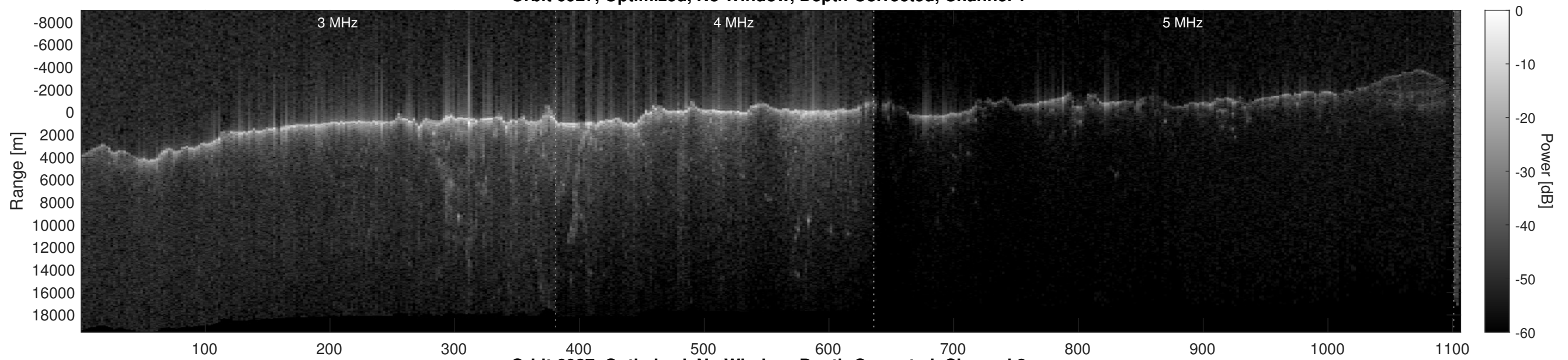
Orbit 6927, Optimized, No Window, Depth-Corrected, Channel 2
