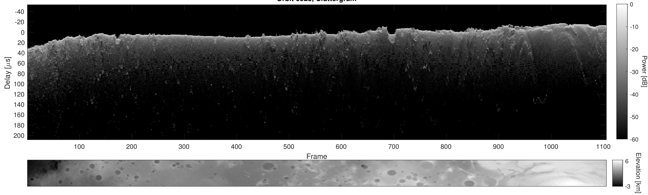
Orbit 6928, Cluttergram
