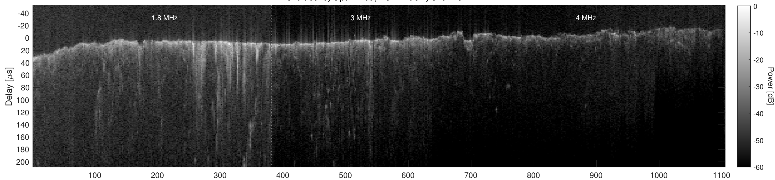
Orbit 6928, Cluttergram
