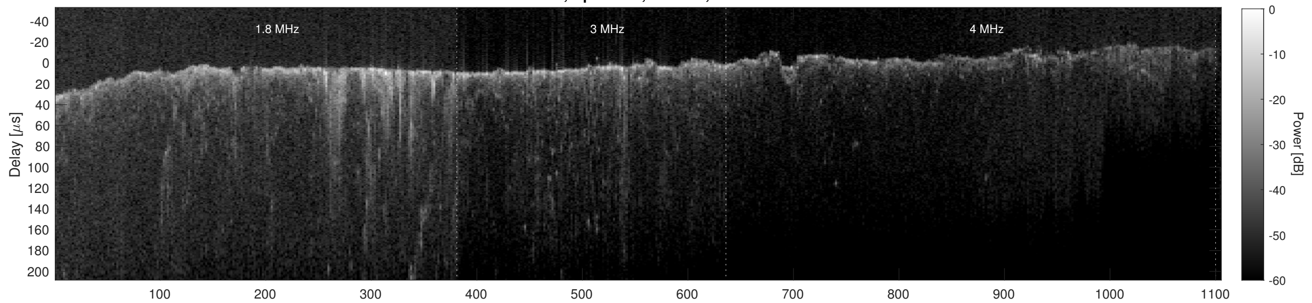
Orbit 6928, Cluttergram
