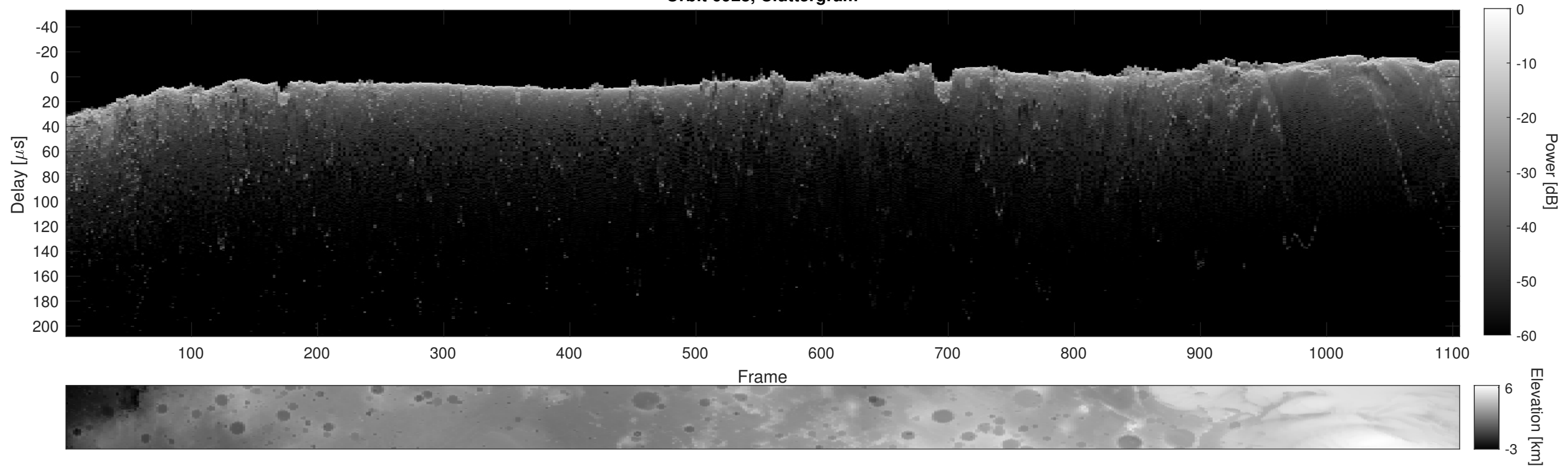
Orbit 6928, Cluttergram
