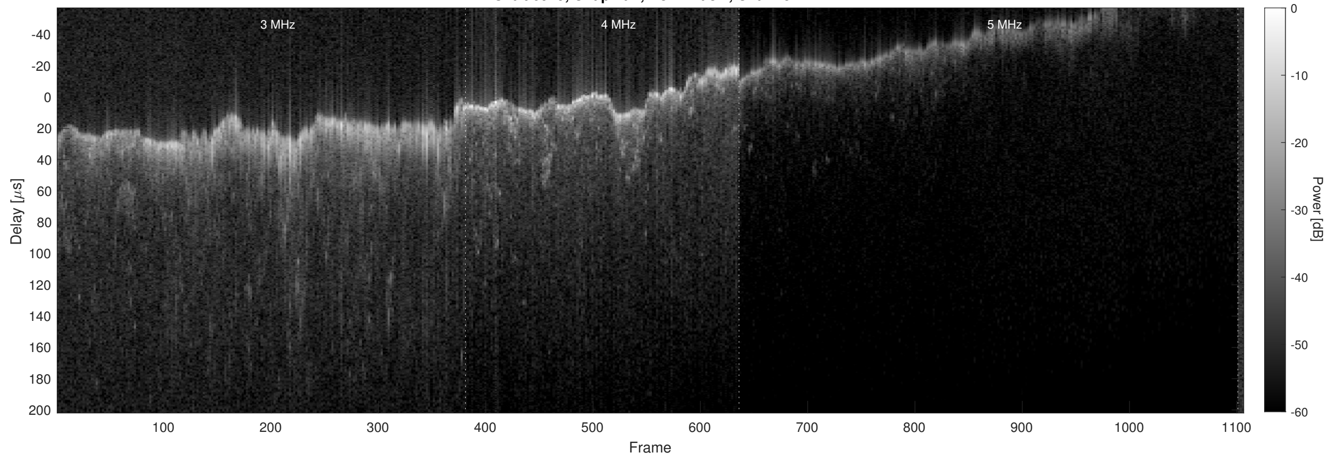
Orbit 6929, Chapman, No Window, Channel 2
