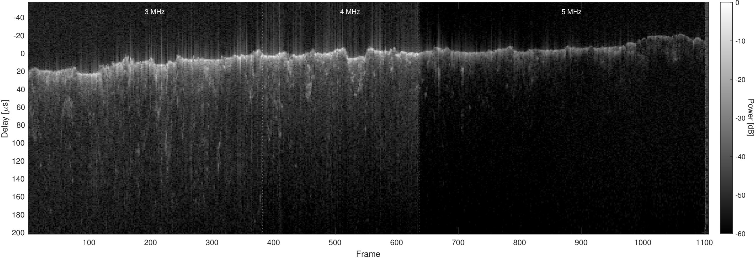
Orbit 6929, Optimized, No Window, Channel 2
