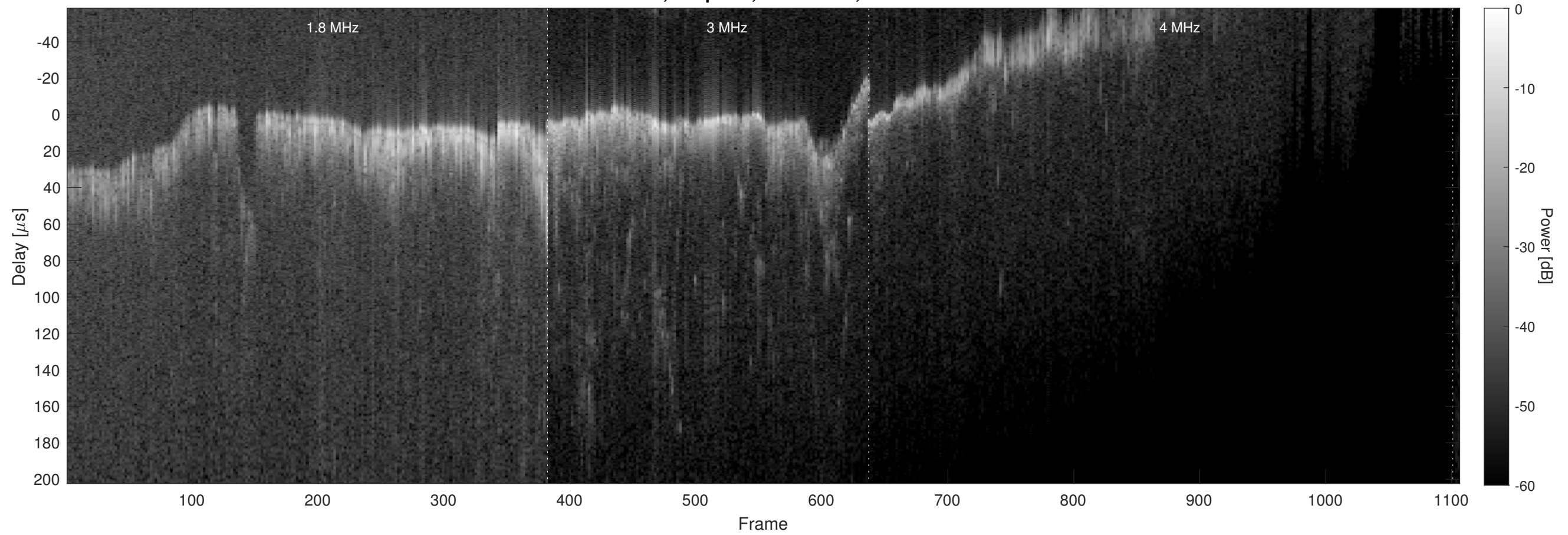
Orbit 6930, Chapman, No Window, Channel 2
