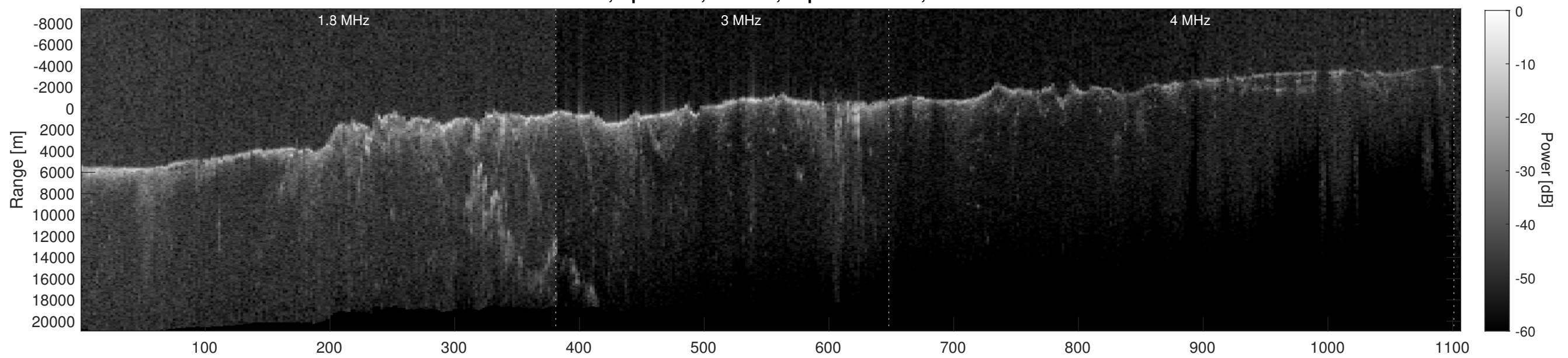
Orbit 6931, Depth-Corrected Cluttergram
