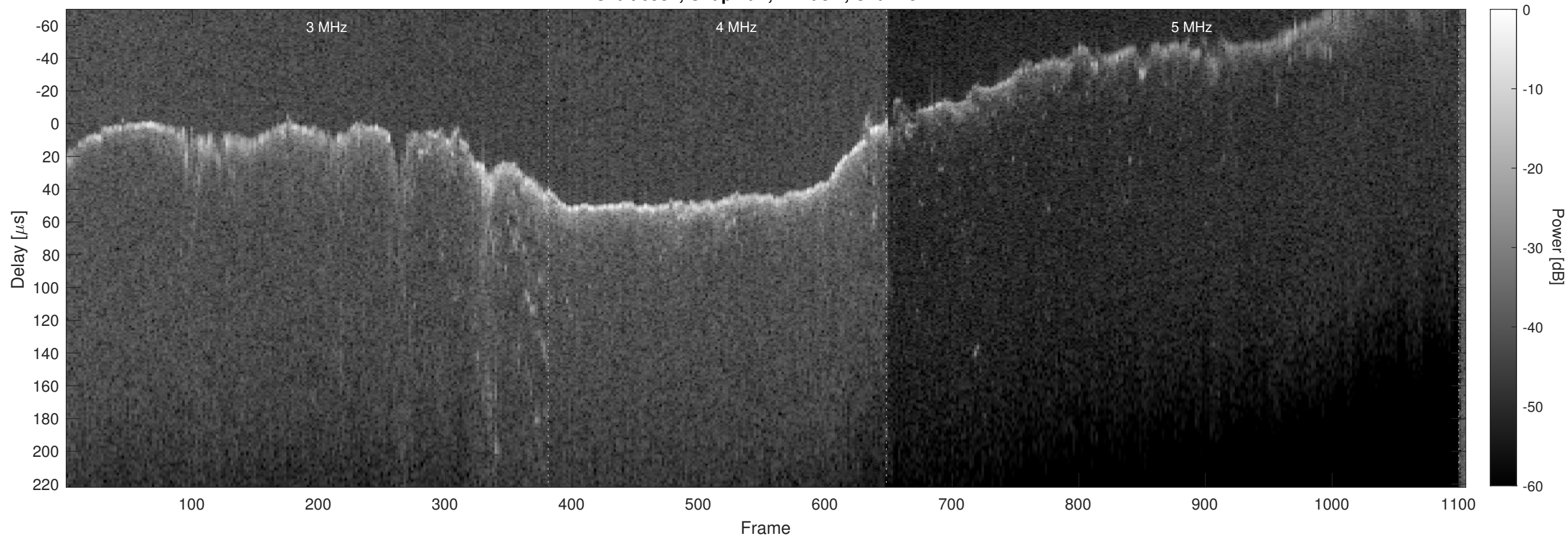
Orbit 6932, Chapman, Window, Channel 2
