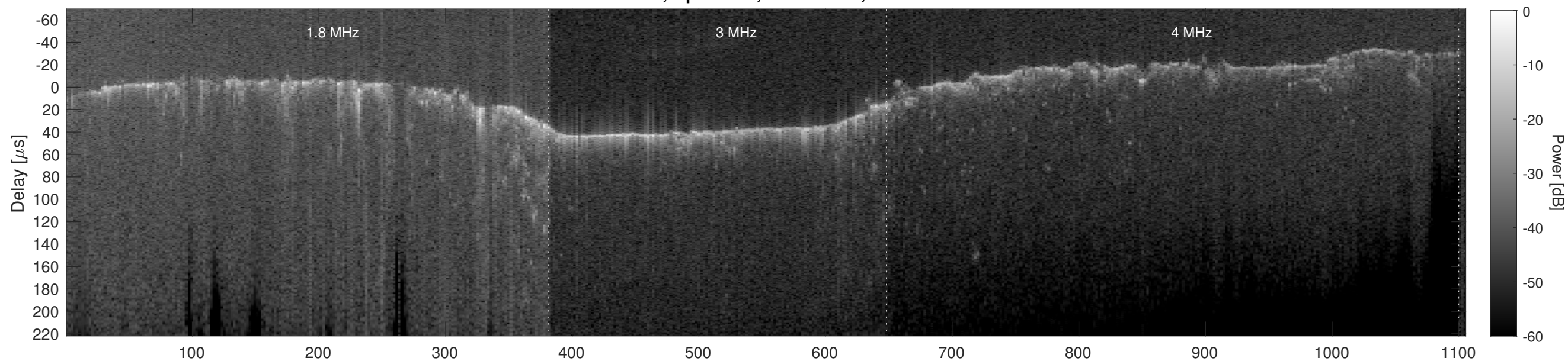
Orbit 6932, Cluttergram
