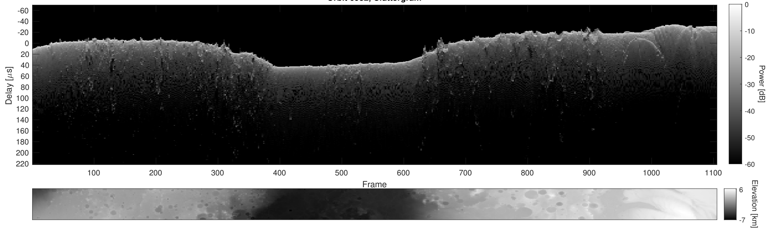
Orbit 6932, Cluttergram
