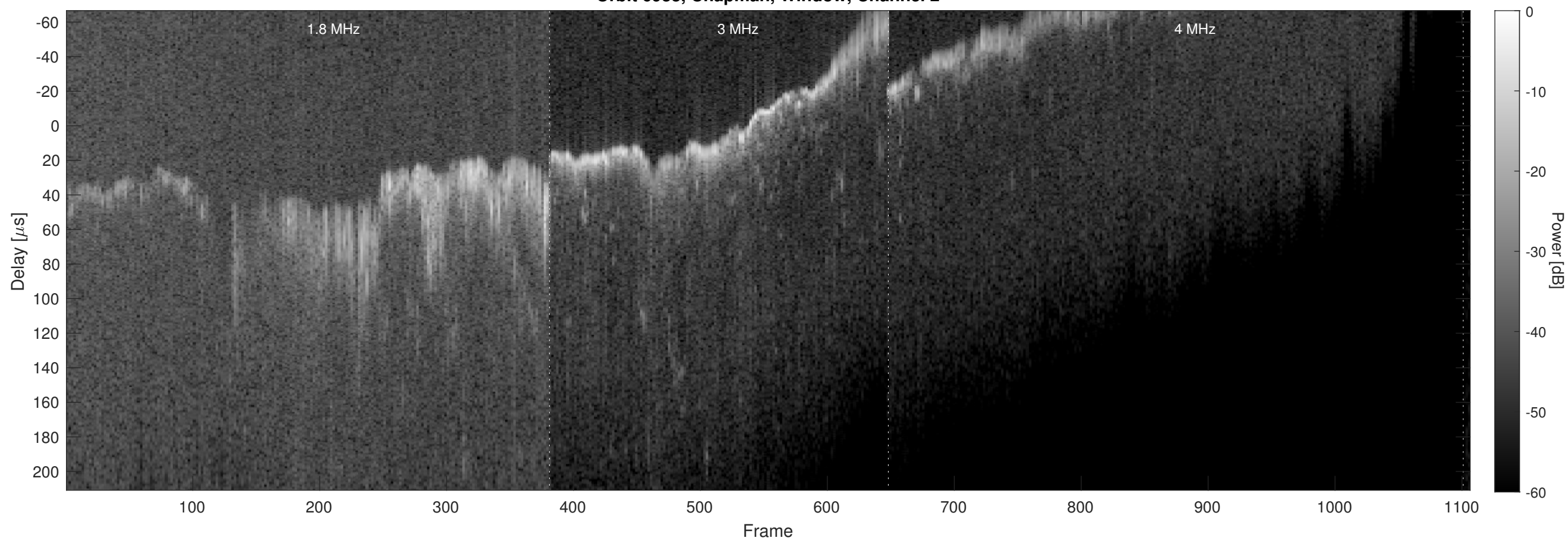
Orbit 6933, Chapman, Window, Channel 2
