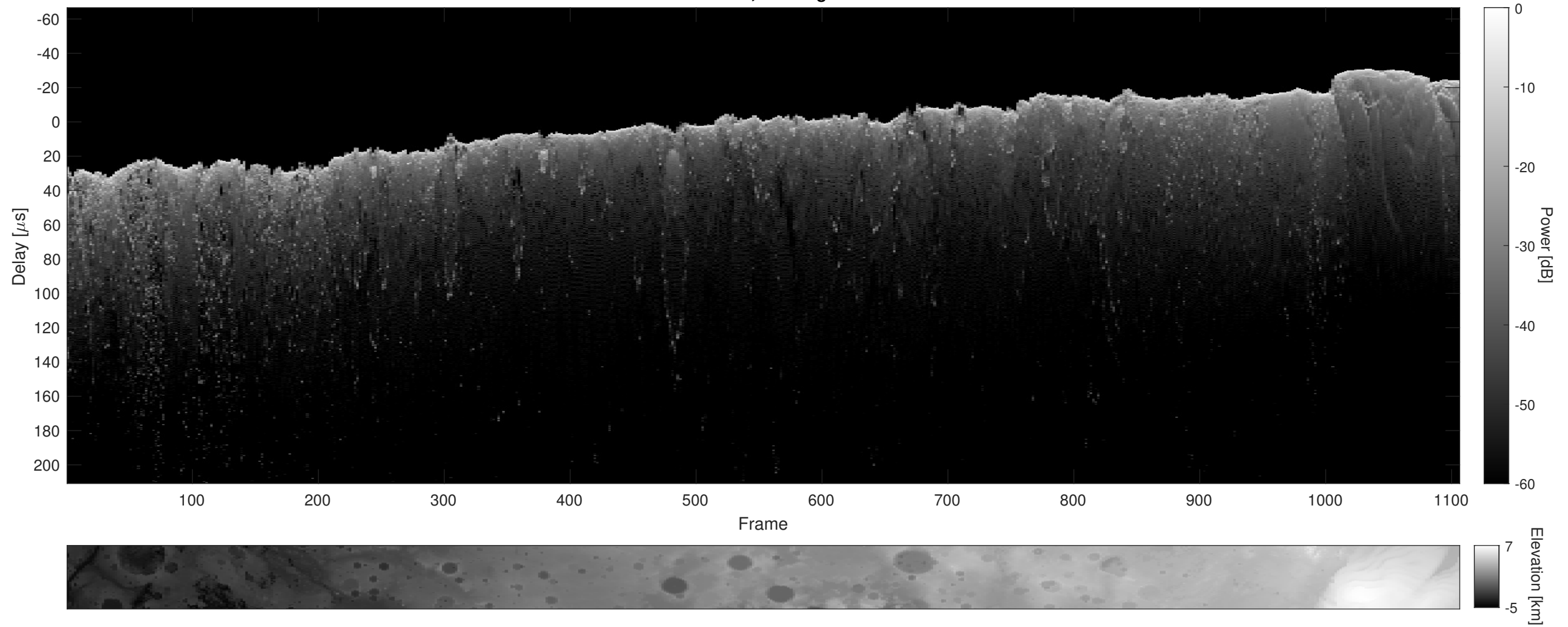
Orbit 6933, Cluttergram
